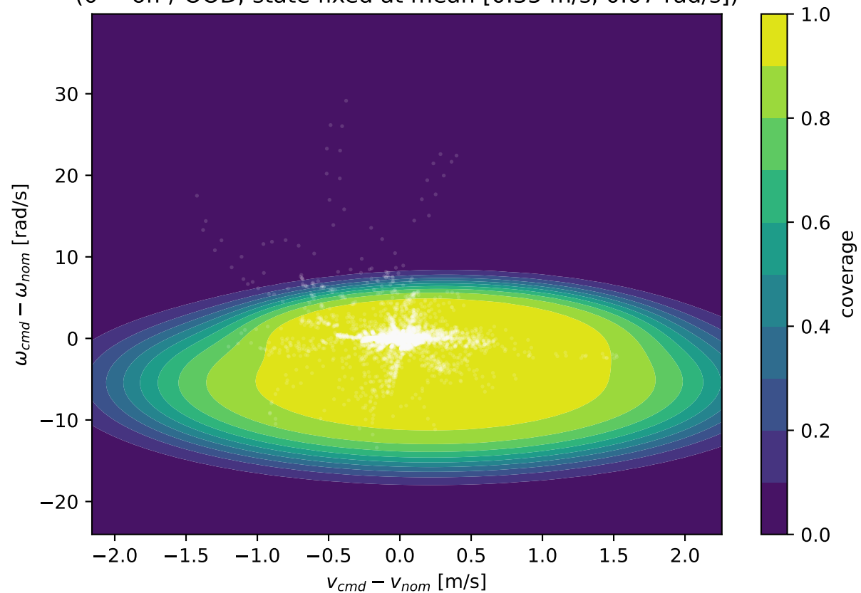
Residual coverage vs command offset (0 = off / OOD; state fixed at mean [0.35 m/s, 0.07 rad/s])
